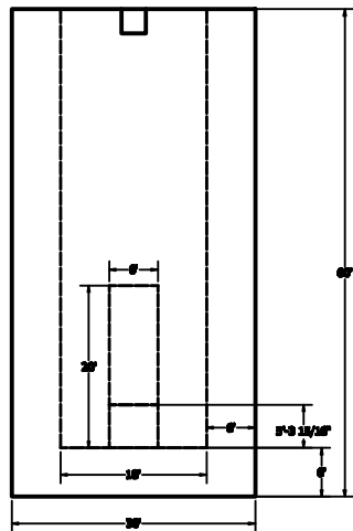
TOP VIEW SCALE 1/320
